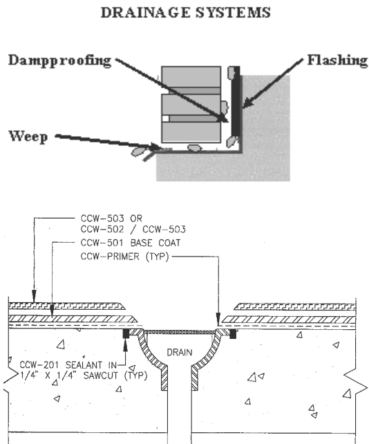
Drainage system for decks
