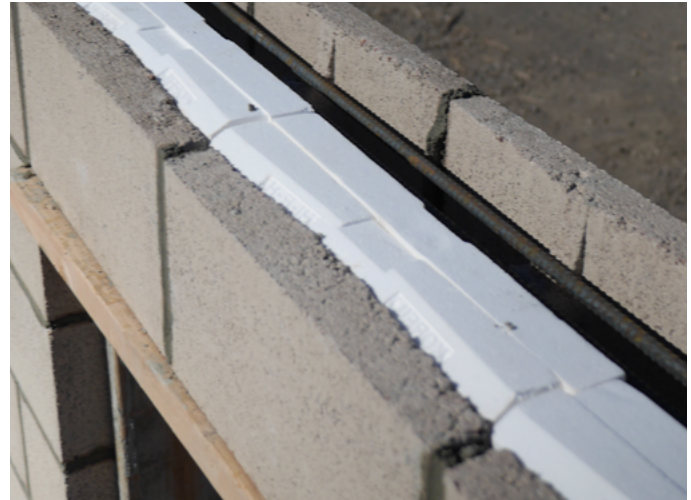
HI-R-H Unit reinforced as a lintel shown prior to grouting
