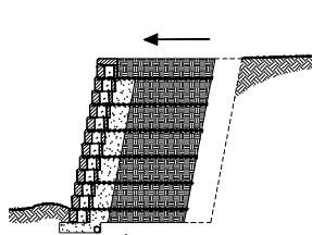
Sliding
