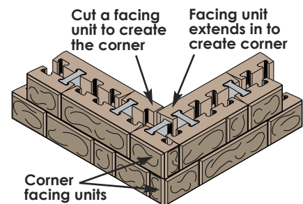
Corner facing units
