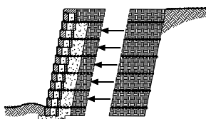
Grid Rupture
