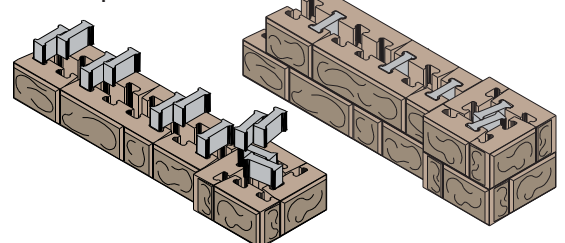
Posts within Parapets
