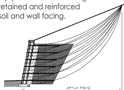
Internal Compound
