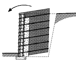
Overturning
