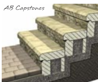
AB Capstone and Pavers
