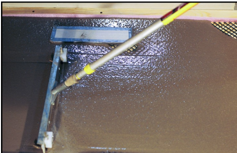
A gauge rake designed for underlayments may be helpful for larger areas
