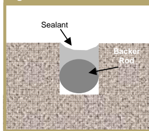
Figure 2: Backer rod
